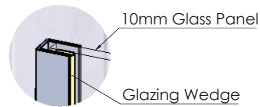
Glass To Wall Tolerance DETAIL A
