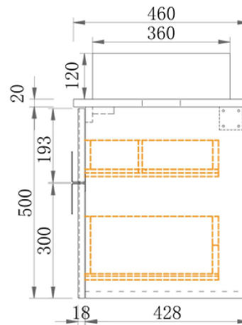
Section Side
