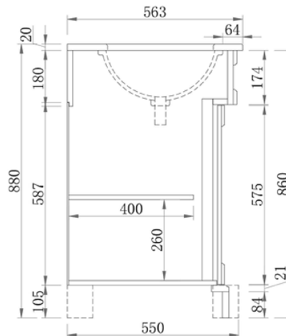
Section Side
