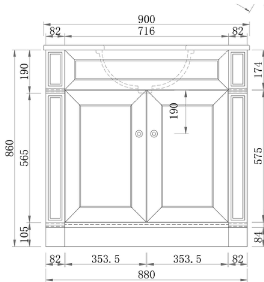
Front Elevation
