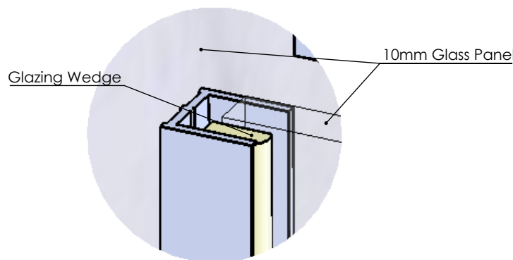
Glass To Wall Tolerance DETAIL A
