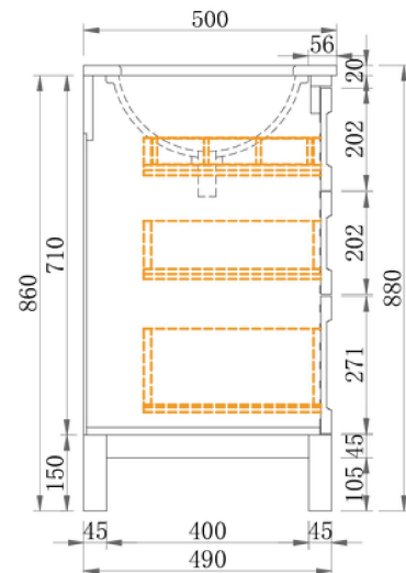
Section Side
