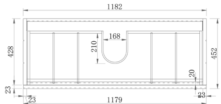
Section Top - Drawer Inserts
