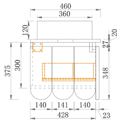
Section Side
