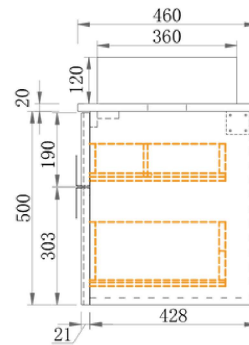
Section Side
