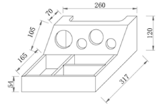
Hairdryer Insert (Lower Drawer)
