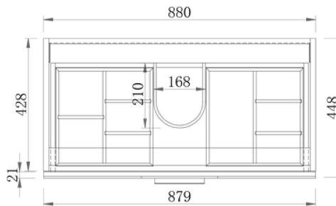
Section Top - Drawer Inserts
