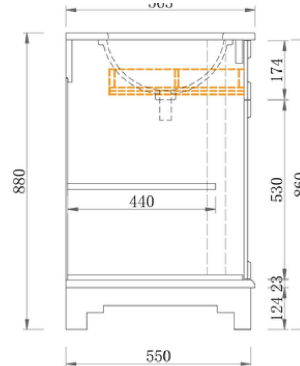
Section Side
