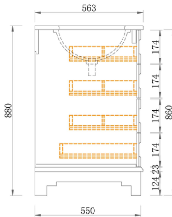
Section Side
