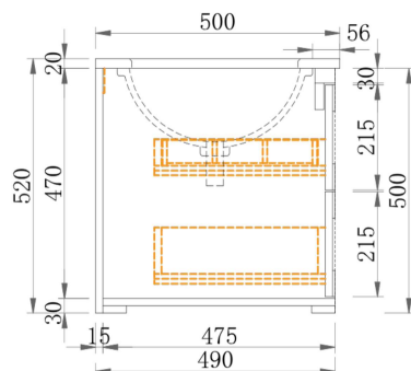
Section Side
