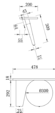
Leg Detail
