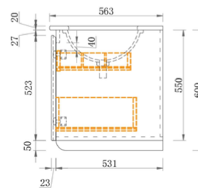
Section Side
